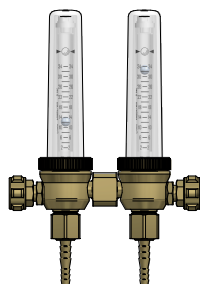
Dual Flowmeter. 34L/min. Art.nr. 37122530
